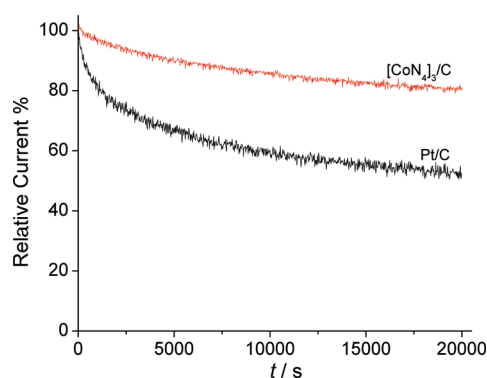
Figure 4. Current–time ( i – t ) chronoamperometric response of [\text{CoN}_4]_3/\text{C} and \text{Pt}/\text{C} modified GC electrode at −0.26 V in \text{O}_2 -saturated aqueous solution of 0.1 M KOH at a rotation rate of 1600 rpm.
