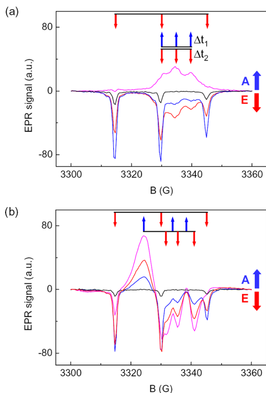
Figure 9. Transient EPR spectra of 1 − (a) and 1 + (b) in CHCl 3 at 280 K, and recorded at increasing time delays after the laser pulse ( t = 0.3, 1.4, 2.7 , and 10.0 \mu\text{s} for magenta, red, blue, and black spectra, respectively). Both spectra were recorded under the same experimental conditions (microwave power, P_{\mu\text{w}} = 10 \text{ mW} ; photoexcitation, \lambda = 532 \text{ nm} ; E/pulse = 5 \text{ mJ} ). The A and E arrows indicate enhanced absorption and emission polarization, respectively. For both peptides, the polarized signals decay to Boltzmann equilibrium within ca. 28 \mu\text{s} .
