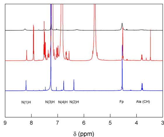
Figure 8. 500 MHz ^1\text{H} NMR in the NH resonance region of 2 mM 1+ and 2+ in \text{CDCl}_3 at room temperature. The spectra correspond (from top to bottom) to 1+ before and after reduction of the nitroxide with 50 equiv of PH, and 2+. N(3)H overlaps the peak of residual chloroform. The peaks at 5.58, 6.85, 7.21, 7.53, and 7.93 ppm belong to PH, which was in excess, and products from its oxidation. 39
