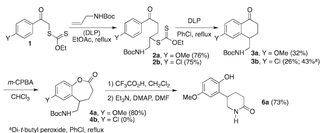
Scheme 2. First Example of an Aryl-piperidone Synthesis
