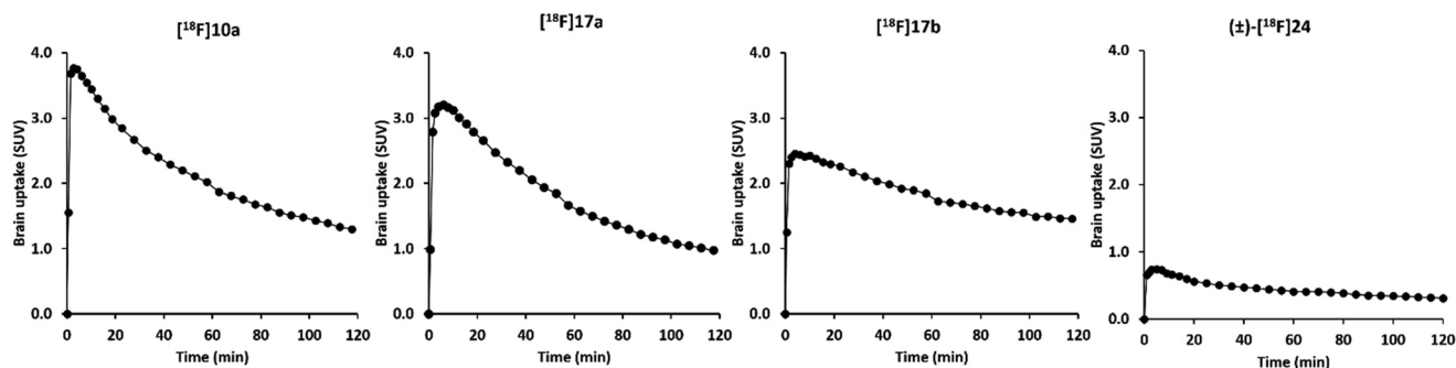
Fig. 2 Representative time-activity curves of microPET studies for [ ^{18}\text{F} ] 10a , [ ^{18}\text{F} ] 17a , [ ^{18}\text{F} ] 17b and (±)-[ ^{18}\text{F} ] 24 in brains of nonhuman primates. The curves indicated that three radiotracers [ ^{18}\text{F} ] 10a , [ ^{18}\text{F} ] 17a and [ ^{18}\text{F} ] 17b achieved the max SUV value fast, at 4–6 min post injection. [ ^{18}\text{F} ] 10a had the highest initial brain uptake while [ ^{18}\text{F} ] 17b exhibited relatively slow washout kinetics. (±)-[ ^{18}\text{F} ] 24 displayed the lowest initial uptake in the brain, indicating it has no capability in penetrating the BBB of nonhuman primate.
