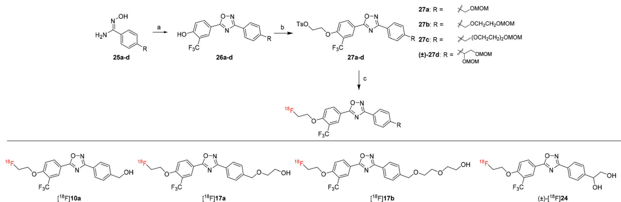
Scheme 6 General syntheses of precursors 27a–d and radiotracers [ ^{18}\text{F} ] 10a , [ ^{18}\text{F} ] 17a , [ ^{18}\text{F} ] 17b , and (±)-[ ^{18}\text{F} ] 24 . Reagents and conditions: (a) 4-Hydroxy-3-(trifluoromethyl)benzoic acid, TBTU, HOBT, DIPEA, DMF, RT–120 °C; (b) ethylene ditosylate, \text{K}_2\text{CO}_3 , \text{CH}_3\text{CN} , 90 °C; (c) [ ^{18}\text{F} ]KF, Kryptofix 222, \text{K}_2\text{CO}_3 , \text{CH}_3\text{CN} , 110 °C, 15 min, 6 N HCl, 5 min.
