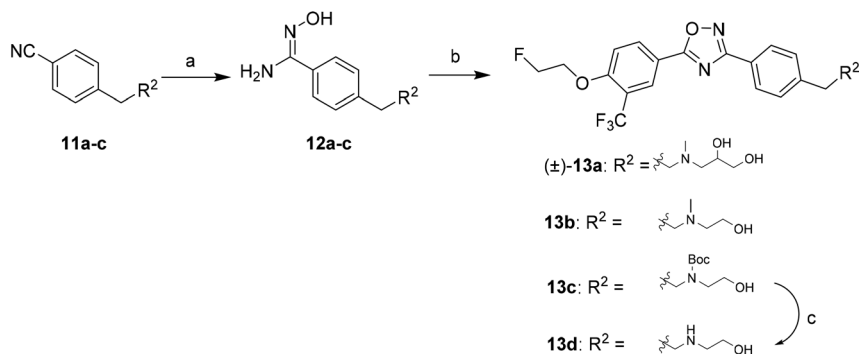
Scheme 2 Syntheses of 13a–d . Reagents and conditions: (a) Hydroxylamine hydrochloride, \text{NaHCO}_3 , methanol, reflux; (b) 9a , TBTU, HOBt, DIPEA, DMF, RT– 120^\circ\text{C} ; (c) 4.0 M HCl in dioxane, RT.
