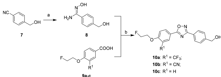
Scheme 1 Syntheses of 10a–c . Reagents and conditions: (a) Hydroxylamine hydrochloride, \text{NaHCO}_3 , methanol, reflux; (b) TBTU, HOBt, DIPEA, DMF, RT– 120^\circ\text{C} .
