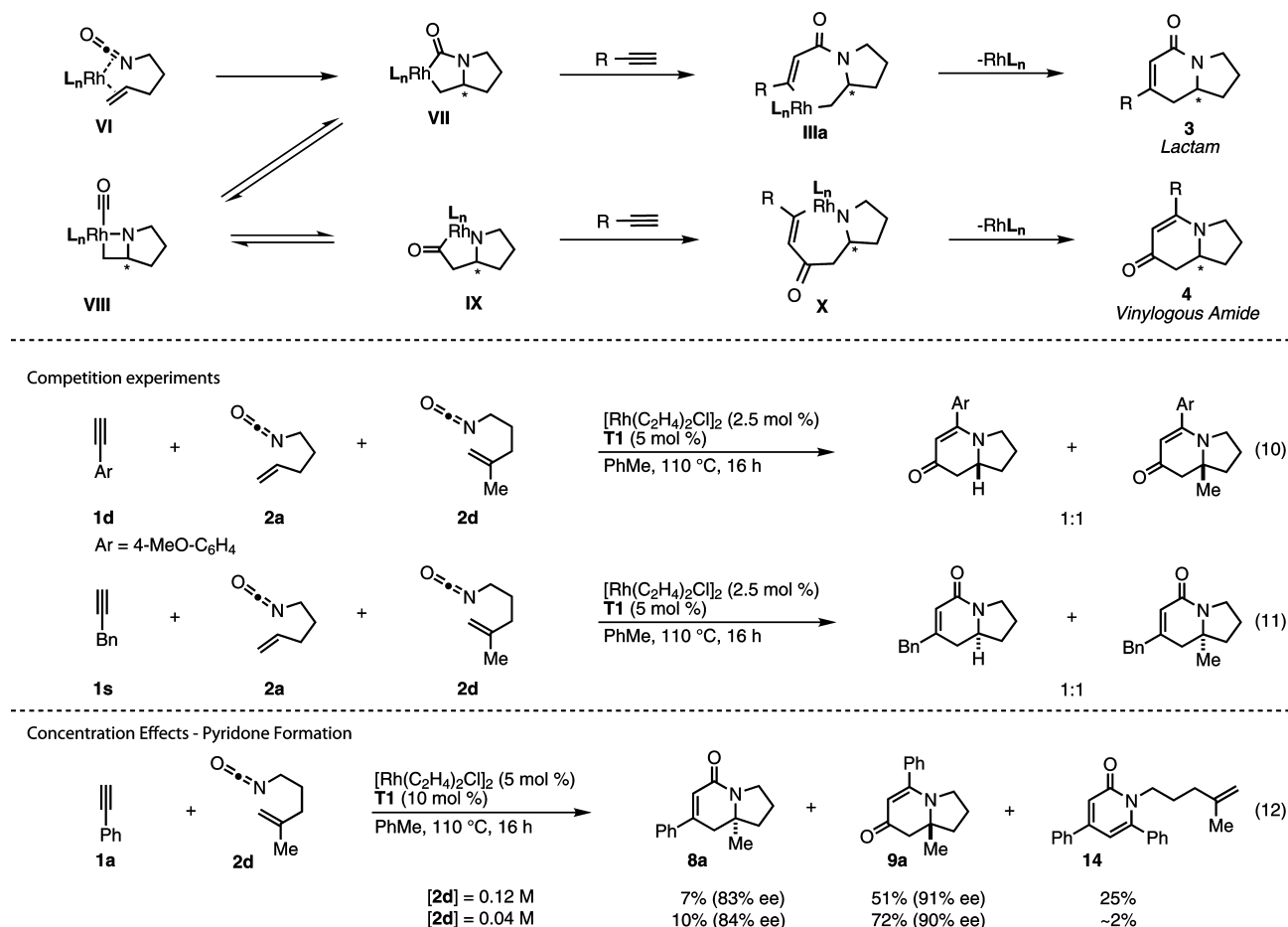
Scheme 3. Alternative Catalytic Cycle
