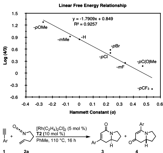
Figure 2. Linear free energy relationship of aryl acetylenes.
