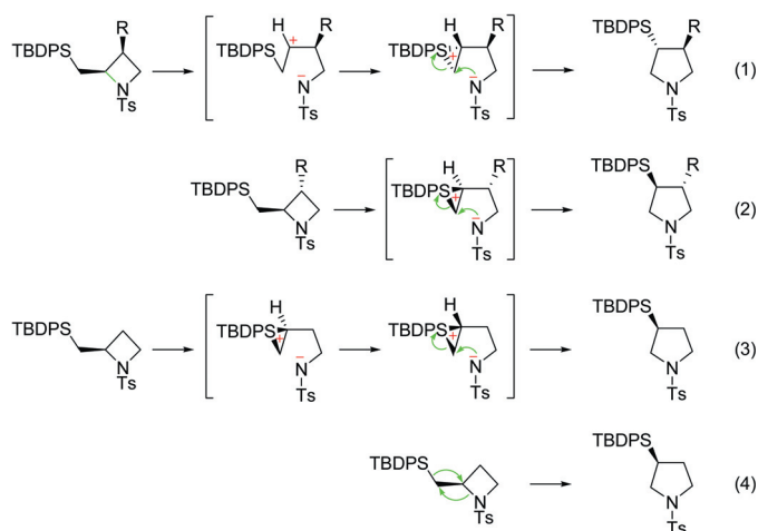
Scheme 4 Mechanistic rationale for the observed enantio-control during azetidine → pyrrolidine rearrangement (both the bonds to silicon in the siliranium ion must be treated as only partial bonds. The use of the full \alpha and \beta bonds are required here to consider the relative stereochemistry of this ring in relation to the substituent R).
