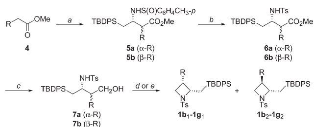
Scheme 2 General protocol for the preparation of N - p -toluenesulfonyl 2- tert -butyldiphenylsilylmethylazetidines: reagents and conditions: (a) (i) LDA, THF, −0 °C (ii) \text{CITi}(\text{i-OPr})_3 , −78 °C (iii) ( S )- tert -BuPh 2 SiCH 2 CH=NS(O)C 6 H 4 CH 3 - p , −78 °C, ~90%; (b) m -CPBA, DCM, 0–25 °C; (c) \text{LiAlH}_4 , THF, 0–25 °C, >90% over the steps (b) and (c); (d) \text{Ph}_3\text{P} , DIAD, C 6 H 6 , 0 °C–rt, >90%; (e) TsCl, KOH, THF, >90%.
