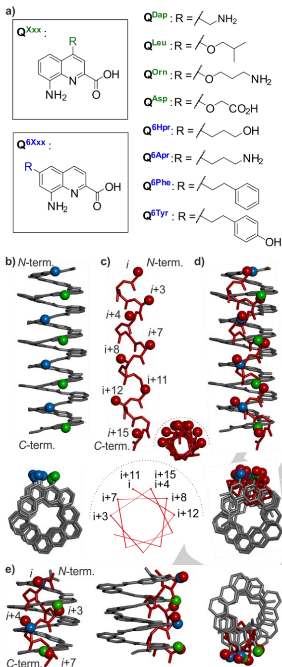
Figure 1. a) Some previously described 4-substituted Q Xxx monomers and some of the new 6-substituted Q Xxx monomers reported in this study. b) Molecular model and helical wheel of a (Q 6Xxx Q Q Xxx Q Q Xxx ) 3 Q 6Xxx Q Q Xxx octadeca-arylhelix showing substituents in position 6 and 4 as blue and green balls, respectively. c) Structure of an ideal (computed) 3.66 13 \alpha -helical hexadecapeptide with \beta -carbons shown as red spheres. d) Overlay of the side chains in b) and c) with an RMSD of 1.50 Å (see Fig. S2). e) Overlay of four side chains of Q 6Xxx Q Q Xxx Q Q Xxx Q 6Xxx (same color code as b) with four side chains of a short 3.6 \alpha -helix (red spheres). Note the position of the side chains in the 3.6 helix slightly differ from those of the 3.66 helix above. An RMSD of 0.92 Å is calculated if the overlay concerns the peptide \beta -carbon and a quinoline exocyclic carbon in position 4 or 6 (shown). An RMSD of 0.79 Å is calculated if the overlay concerns the peptide \alpha -carbon and the quinoline endocyclic carbon in position 4 or 6 (not shown).
