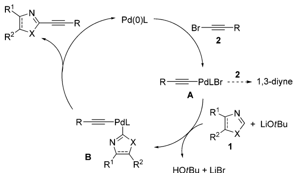
Scheme 1. Plausible Mechanism of the Pd-Catalyzed Direct Alkyynylation of Heterocycles
