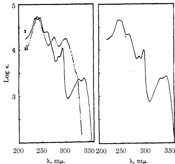
Fig. 2.—I, 2-nitrodibenzalcohol: I, dibenzothiophene; II, dibenzoselenophene.
