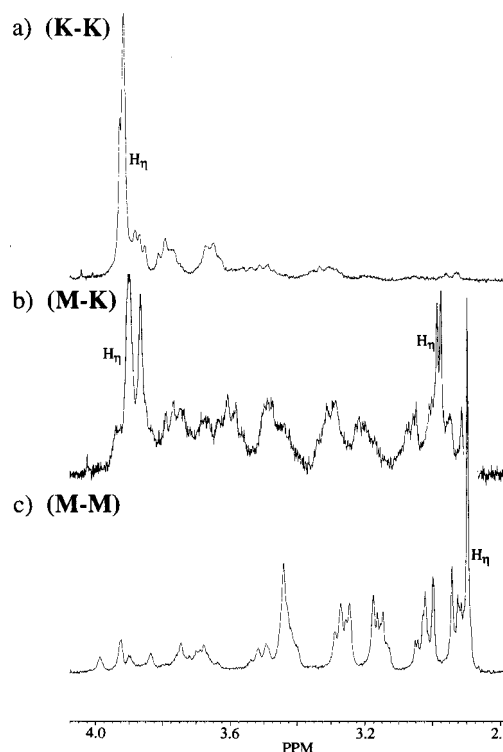
Figure 9. 1 H NMR spectra (3–4 ppm region) at 400 MHz in CD 2 Cl 2 of the dimers, K-K, K-M, and M-M.
