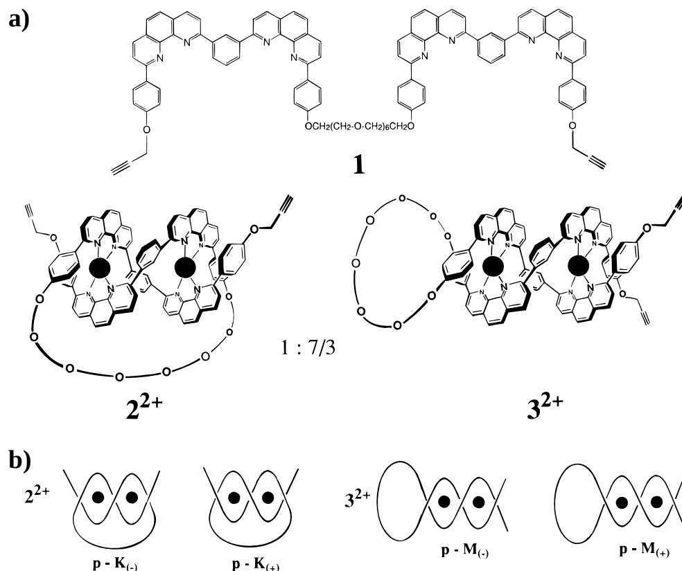
Figure 3. (a) The two helicoidal dicopper(I) precursor complexes: pre-knot 2^{2+} and pre-macrocycle 3^{2+} . (b) Schematic representation of their enantiomers.
