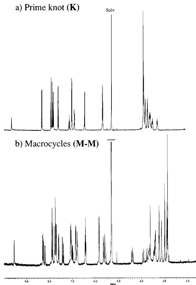
Figure 8. 1 H NMR spectra at 400 MHz in CD 2 Cl 2 of the prime knot K ( 9 2+ ) and the M-M dimer family (complexes 12 4+ , 13 4+ ).
