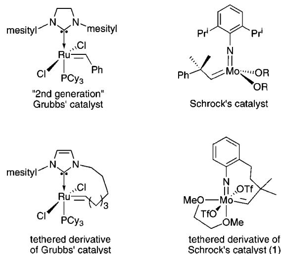
Scheme 1. Previous Tethered Alkylidene Synthesis
