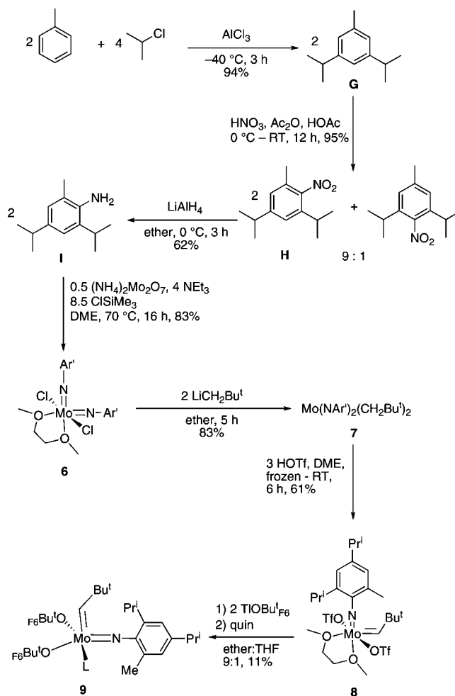
Scheme 4. Synthesis of \text{Mo}(\text{OBu}^t\text{F}_6)_2(\text{NAr}')(\text{=CHBu}^t)(\text{quin}) ( 9 )
