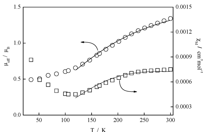
Figure 6. Plot of \mu_{\text{eff}} and \chi_M (per Cu) vs temperature for complex C1 . The solid lines were calculated using the parameter set given in the text and are restricted to the 100–300 K region since this is the region sensitive to J .
