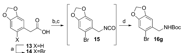
Scheme 3 Synthesis of piperonyl cyclisation precursor 16g . Reagents and conditions: (a) DBDMH, 4 M NaOH, H 2 O, rt, 16 h, 91%; (b) dppe, Et 3 N, CH 2 Cl 2 , 0 °C → rt, 0.5 h; (c) (i) silica plug filtration (partial conversion); (ii) PhMe, 110 °C, 1 h (complete conversion); (d) t BuOH, 80 °C, 16 h, 50% over 3 steps.
