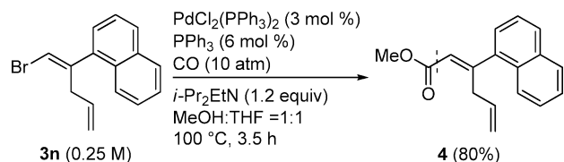
Scheme 3. Three-Component Processes with the Subsequent Pd-Catalyzed Reactions
