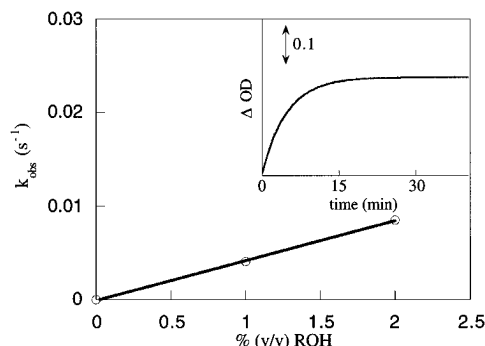
Figure 1. Dependence of k_{\text{obs}} for formation of \text{Cu(dmp)}_2^+ on methanol concentration in dichloromethane at 25 °C ( P_{\text{NO}} = 1 atm). Inset: representative kinetic trace and its first-order fit.
