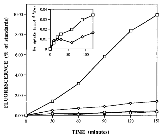
Figure 4. Appearance of anthracene fluorescence ( \lambda_{\text{exc}} = 375 \text{ nm} , \lambda_{\text{em}} = 415 \text{ nm} ) in the culture media of Pseudomonas putida JM218 upon treatment with labeled ferrichrome analogs 5G and 5A in the absence ( 5G , \square ; 5A , \diamond ) and presence ( 5G , \circ ; 5A , \triangle ) of \text{NaN}_3 as inhibitor. Insert: {}^{55}\text{Fe} uptake with the ferrichrome analogs 5G ( \square ) and 5A ( \diamond ).
