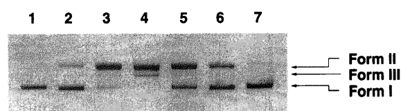
Fig. 6. Photochemical Cleavage of pBR322 Plasmid DNA by 13
