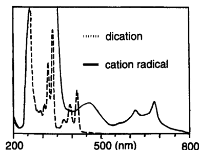
Fig. 2. UV Spectra of 13
