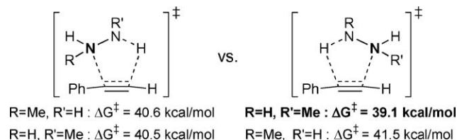
Fig. 1 Calculated activation energies associated with the four possible hydroamination TS. 8
