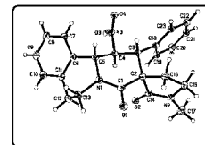
X-ray structure of 1a
