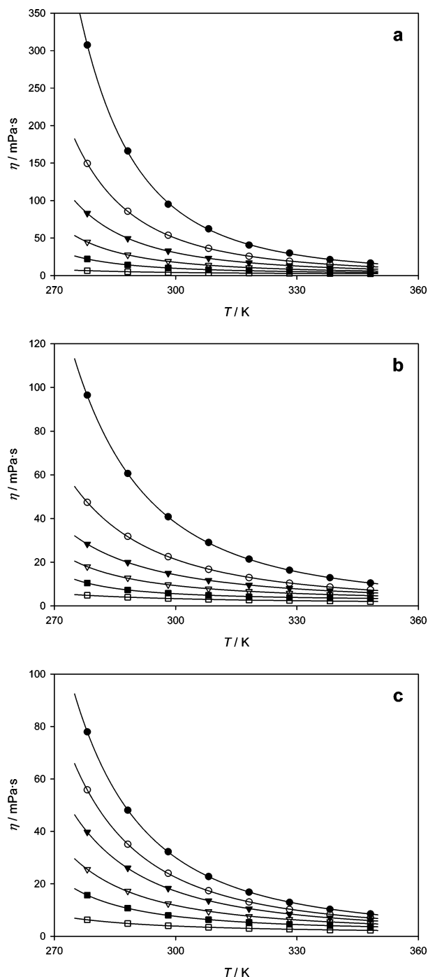
Figure 2. Dynamic viscosity \eta for the water (1) + IL (2) binary systems as a function of temperature at different approximated mass fractions of water: \bullet , 0 %; \circ , 2 %; \blacktriangledown , 5 %; \nabla , 10 %; \blacksquare , 20 %; \square , 50 %. The correlations performed with the VFT equation are plotted as solid lines. IL: (a) [emim][EtSO 4 ]; (b) [emim][OTf]; (c) [emim][TFA].
