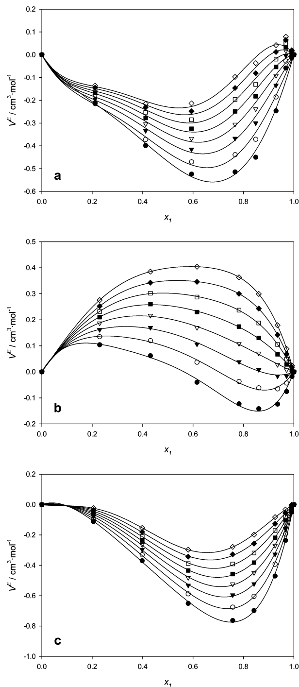
Figure 4. Excess molar volume V^E for the water (1) + IL (2) systems at different temperatures: \bullet , 278.15 K; \circ , 288.15 K; \blacktriangledown , 298.15 K; \nabla , 308.15 K; \blacksquare , 318.15 K; \square , 328.15 K; \blacklozenge , 338.15 K; \diamond , 348.15 K. The solid lines represent the corresponding correlations by the Redlich–Kister equation. IL: (a) [emim][EtSO 4 ]; (b) [emim][OTf]; (c) [emim][TFA].
