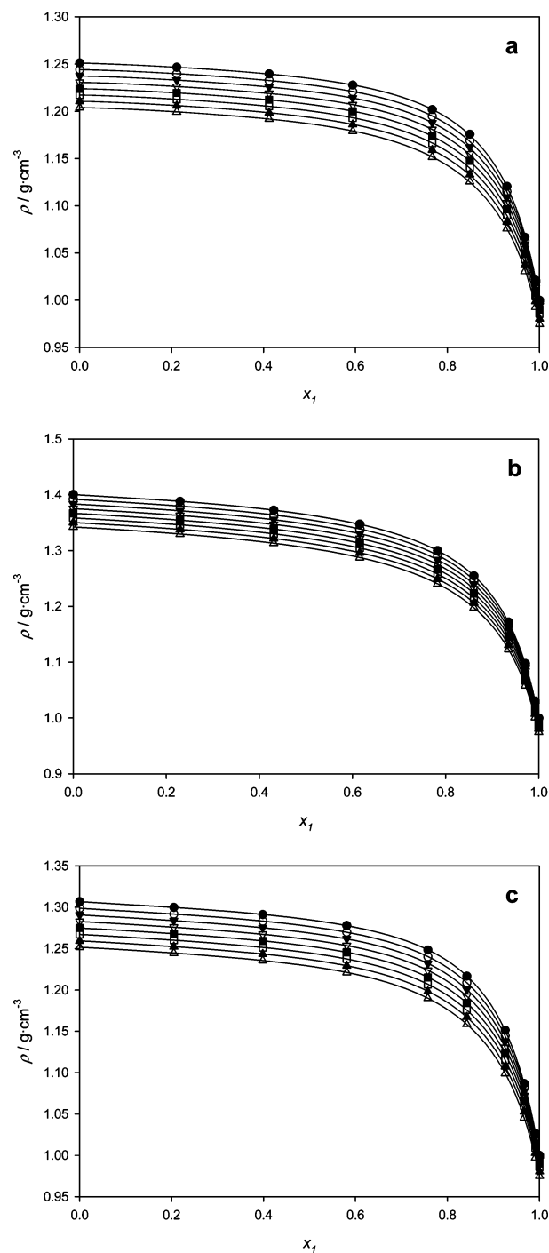
Figure 6. Density \rho for the water (1) + IL (2) systems, as a function of mole fraction of water, at different temperatures: ●, 278.15 K; ○, 288.15 K; ▼, 298.15 K; ▽, 308.15 K; ■, 318.15 K; □, 328.15 K; ▲, 338.15 K; △, 348.15 K. The solid lines correspond to the fits derived from the Redlich–Kister correlation of the excess molar volume V^E . IL: (a) [emim][EtSO 4 ]; (b) [emim][OTf]; (c) [emim][TFA].
