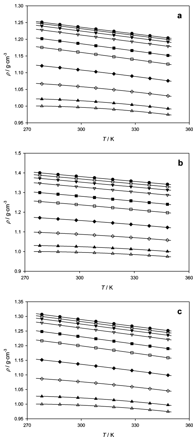
Figure 1. Density \rho for the water (1) + IL (2) binary systems as a function of temperature at different approximated mass fractions of water: \bullet , 0 %; \circ , 2 %; \blacktriangledown , 5 %; \nabla , 10 %; \blacksquare , 20 %; \square , 30 %; \blacklozenge , 50 %; \diamond , 70 %; \blacktriangle , 90 %; \triangle , 100 %. Polynomial correlations are plotted as solid lines. IL: (a) [emim][EtSO 4 ]; (b) [emim][OTf]; (c) [emim][TFA].
