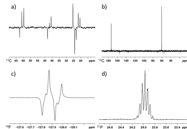
Figure 6 a) SABRE-Relay hyperpolarized ^{13}\text{C} spectrum of 3-methyl-1-butanol, b) SABRE-Relay hyperpolarized ^{13}\text{C} spectrum of methyl glycolate, c) SABRE-Relay hyperpolarized ^1\text{H} - ^{19}\text{F} INEPT spectrum of 2,2-difluoroethanol, d) SABRE-Relay hyperpolarized ^{31}\text{P} spectrum of diethyl (hydroxymethyl) phosphonate. Corresponding thermally polarised spectra are available in the supporting information.
