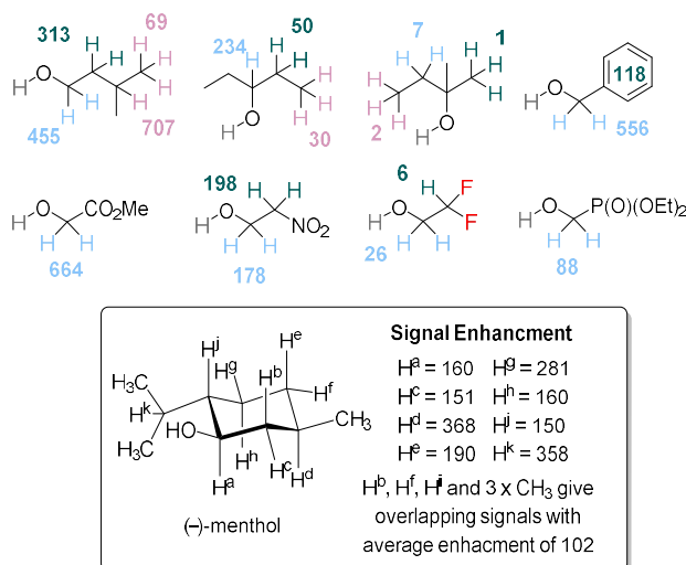
Figure 5 ^1\text{H} NMR per proton signal gains for structurally diverse alcohols at 9.4 T. NMR assignments of (–)-menthol were made by comparison to literature data. 57
