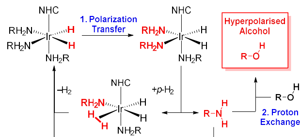
Scheme 1. The SABRE-Relay catalytic cycle for hyperpolarization for alcohols. Polarization is initially transferred from the p\text{-H}_2 derived hydride ligands to a carrier amine ( \text{RNH}_2 ) which subsequently transfer polarization to the alcohol via proton exchange. NHC is N -heterocyclic carbene.
