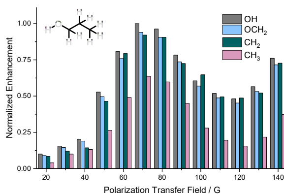
Figure 2. Normalized 1 H NMR signal enhancements in propanol achieved using BnNH 2 as the SABRE-Relay agent as a function of the size of the polarization transfer field.
