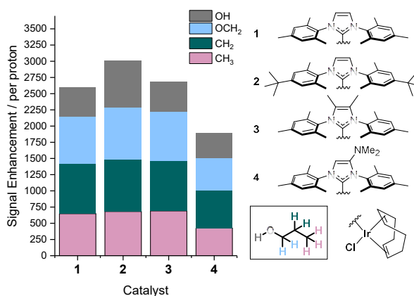
Figure 3. Structures of catalysts 1-4 and the resulting 1 H NMR signal enhancements per proton they deliver to 1-propanol at 9.4 T after SABRE-Relay transfer from NH 3 . Enhancements for each proton environment are characterized by the height of each individual colour bar.
