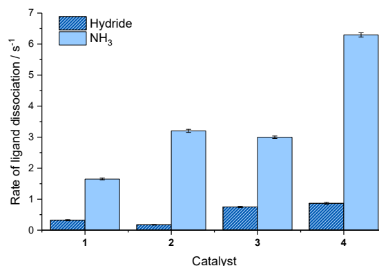
Figure 4. Effective rates of ligand dissociation ( \text{s}^{-1} ) from the corresponding SABRE catalyst at 298 K as measured by EXSY spectroscopy.
