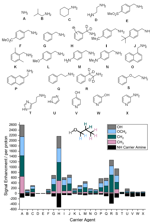
Figure 1. (top) Structures of carrier agents A–X screened for SABRE-Relay polarization of 1-propanol and the resulting 1 H NMR signal enhancements within the spin system per proton at 9.4 T they achieve (bottom). Enhancements for each proton environment are characterized by the height of each individual colour bar.
