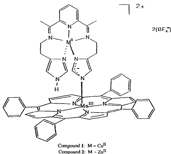
Fig. 1. Schematic representation of the imidazolate-bridged binuclear manganese(III) porphyrin compounds (M II = Cu, Zn).
