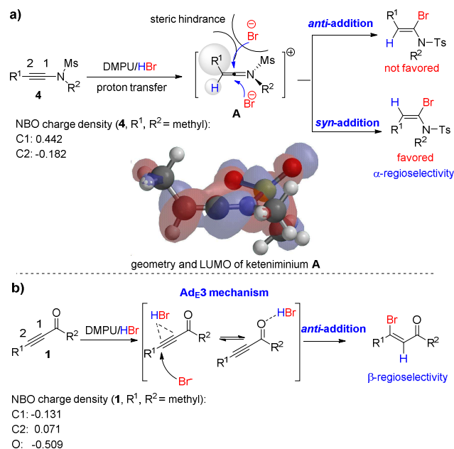
Scheme 4. Proposed mechanism. LUMO of keteniminium was calculated at B3LYP/6-311+G(2df,2p) level of theory.
