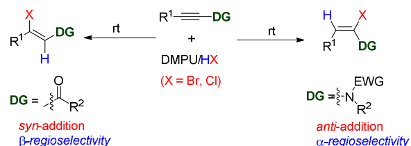
Scheme 1. Halogenation of ynones and ynamides.
