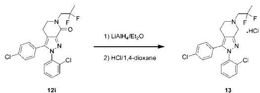
Figure 2. Preparation of amino analogue 13 .
