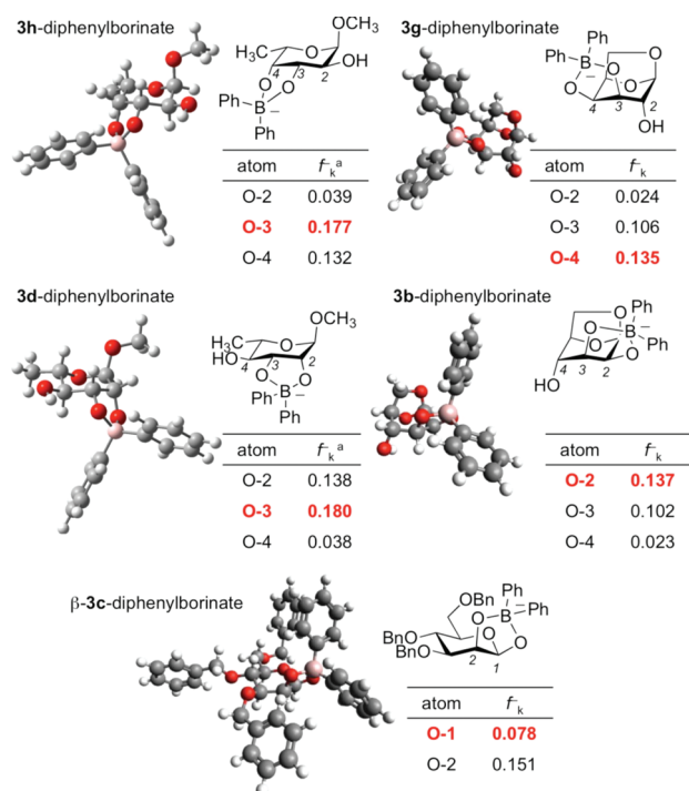
Figure 1. Calculated structures and condensed Fukui indices (B3LYP/6-311+G(d,p)) of diphenylborinates of 3b – 3d , 3g , and 3h . The site of observed reactivity under the catalytic reaction conditions is indicated in bold type (red color). a From ref 11.
