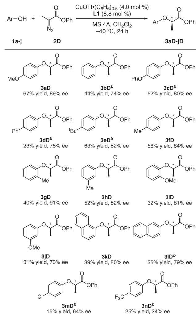
Scheme 1. Scope of Phenols ( 1 ) in the Asymmetric Copper-Catalyzed Carbenoid Insertion with 2D a
