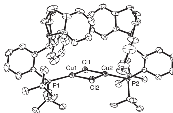
Figure 2. ORTEP drawing of the crystal structure of CuCl(L1) . The hydrogen atoms and the solvent molecule (Et 2 O) have been omitted for clarity.
