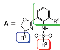
Figure 2. Generic structure of sulfonamide A .
