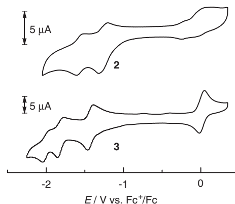
Figure 4. Cyclic voltammograms of 2 (top) and 3 (bottom) in CH_2Cl_2 with 0.1 M n-Bu_4NClO_4 . The data were obtained using a glassy-carbon working electrode and Ag/AgCl reference electrode at a scan rate of 100 mV s −1 .
