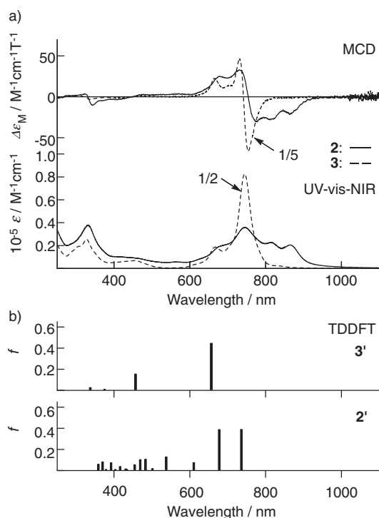
Figure 2. a) MCD and electronic absorption spectra of 2 (solid line) and 3 (broken line) measured in CHCl_3 . b) Calculated absorption stick spectra of 2' and 3' (B3LYP/6-31G*).
