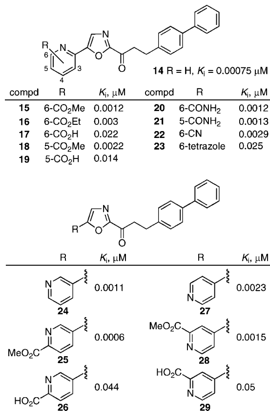
Figure 5. Effect of pyridyl derivatives.
