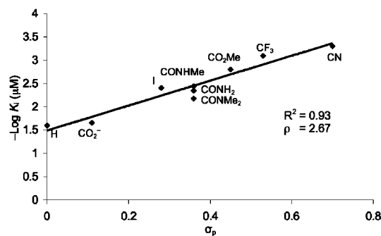
Figure 9. Plot of -\log K_i ( \mu M) versus \sigma_p for 4-(phenoxyethyl)phenethyl series.
