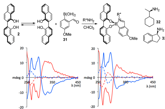
Figure 3. Three-component assembly with 2 and 31 . Left: CD spectra of the reaction products obtained using 2 , 31 , and (R)- 32 (solid blue) or (S)- 32 (solid red). The spectra shown with dashed lines correspond to the condensation products of 31 with (R)- 32 (dashed blue) or (S)- 32 (dashed red) in the absence of 2 . Right: The same comparison was performed with amine 33 . Concentrations were 3.75 \times 10^{-5} M in CHCl 3 .
