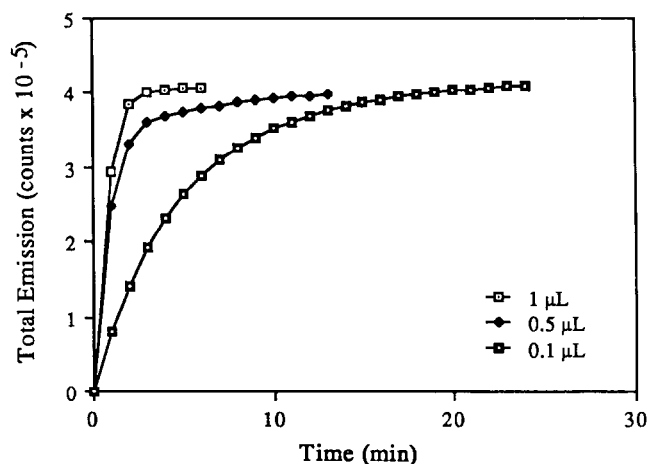
Figure 1. Plot of total chemiluminescence from alkaline phosphatase triggering of dioxetane 2 at pH 10.3 with 1, 0.5, and 0.1 \mu\text{L} of phosphatase suspension.
