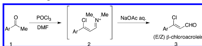
Scheme 1. Preparation of \beta -chloroacroleins using POCl 3 and DMF as VR precursors
