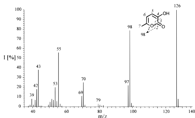
Figure 6. Mass spectrum (MS/EI) of 3-hydroxy-6-methyl-2(2H)-pyranone.
