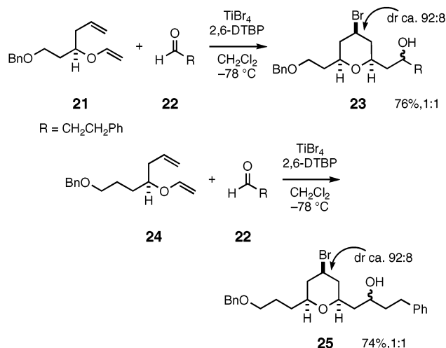
Scheme 3. MAP Cyclizations with O -Benzyl Enol Ether Components
