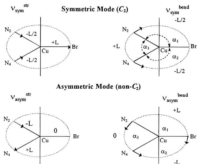
Figure 5. Symmetric and asymmetric modes of vibration for the five coordinate \text{CuN}_4\text{Br} chromophore, including the relative magnitudes ( L ). 2,6
