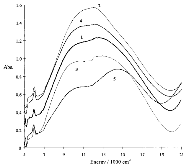
Figure 8. Electronic reflectance spectra of some [\text{Cu}(\text{phen})_2\text{Br}][\text{Y}] complexes.
