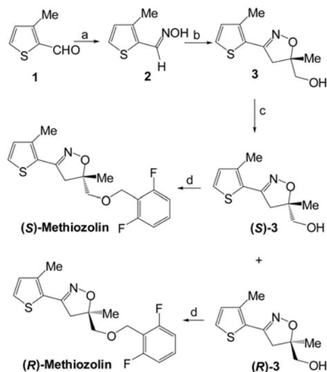
Scheme 1. Synthesis of enantiopure methiozolins.
