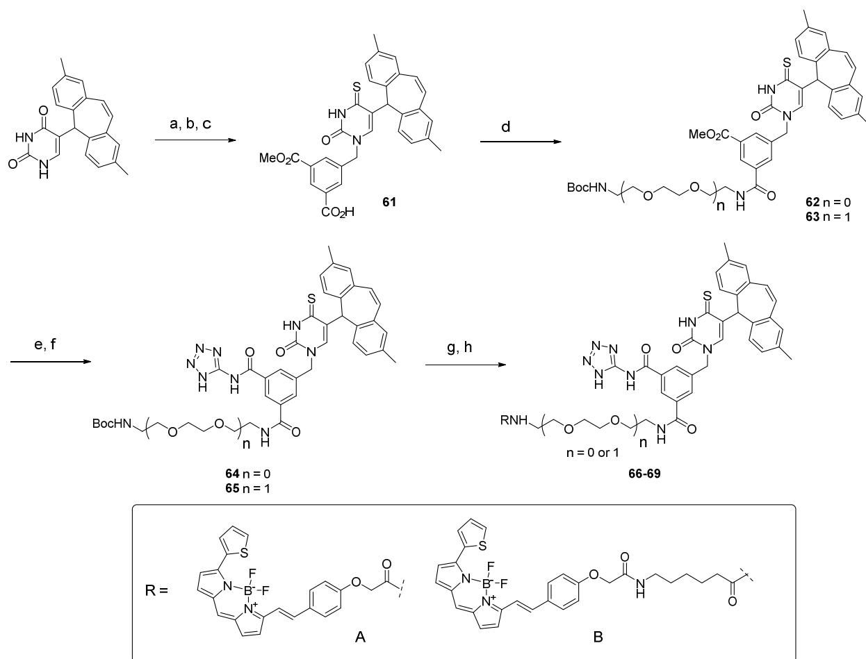
Scheme 4. a) Dimethyl 5-(bromomethyl)isophthalate, BSTFA, 1,2-dichloroethane, reflux, 16 h. b) Lawesson's reagent, 1,4-dioxane, reflux, 16 h. c) 2eq NaOH, MeOH, toluene, H 2 O, 4h. 65% (3 steps) d) tert -butyl (2-(2-aminoethoxy)ethyl)carbamate (53%) or tert -butyl (2-aminoethyl)carbamate (63%), NEt 3 , benzotriazol-1-yl-oxytripyrrolidinophosphonium hexafluorophosphate, DMF, rt, 0.5 h. e) LiOH, MeOH, H 2 O, 16 h, rt. 14-30%. f) 4-aminotetrazole, NEt 3 , Benzotriazol-1-yl-oxytripyrrolidinophosphonium hexafluorophosphate, DMF, 1h, rt. g) 4M HCl in 1,4-dioxane, 1h. h) bodipy-SE, DIPEA, DMF, rt, 1-4 h. 15-45%.
