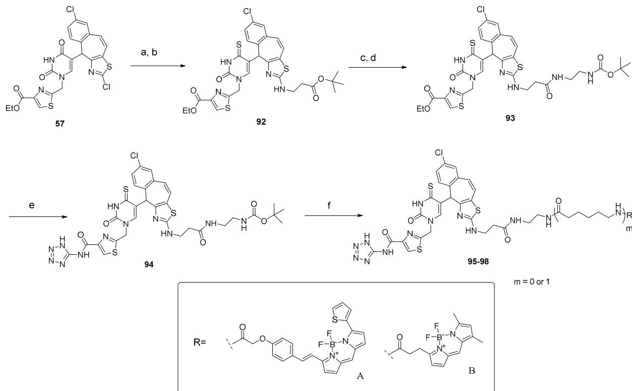
Scheme 6. Reagents and conditions: (a) amine, NEt 3 , 1,4-dioxane, reflux, 72 h. (89%). (b) Lawesson's reagent, 1,4-dioxane, reflux, 18 h (48%). (c) TFA, DCM, rt, 30 min (55%). (d) tert -butyl (2-aminoethyl)carbamate, HATU, DCM, DIPEA, rt, 24 h (63%). (e) 1. NaOH, MeOH, reflux, 4 h; 2. 5-aminotetrazole, Benzotriazol-1-yl-oxytripyrrolidinophosphonium hexafluorophosphate, DIPEA, DMF, rt 4 h (28% over 2 steps). (f) 1. TFA, DCM, rt, 30 min; 2. bodipy-SE, DIPEA, DMF, rt, 1-4 h. (11-18%, 2 steps). The structures of compounds 95-98 are assigned in table 6.
