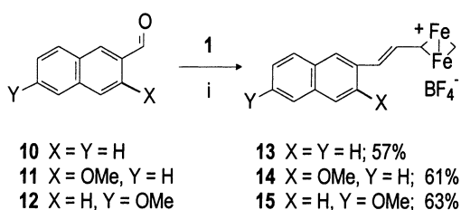
Scheme 5. Reagents and conditions: (i) \text{CH}_2\text{Cl}_2 , reflux, 12 h.
