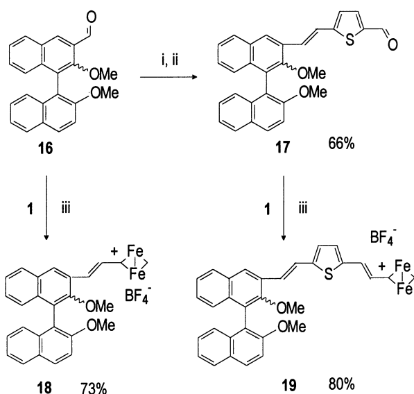
Scheme 6. Reagents and conditions: (i) Diethyl(2-thienylmethyl)phosphonate, \text{KO}^t\text{Bu} , THF, 1 h; (ii) \text{BuLi} , THF, -78^\circ\text{C} , 1 h. DMF, 30 min; (iii) \text{CH}_2\text{Cl}_2 , reflux 18 h.
