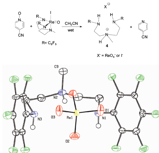
Figure 8. X-ray single crystal structure [(\text{C}_6\text{F}_5)(\text{NHCH}_2\text{CH}_2)_2\text{HN}(\text{Me})][\text{ReO}_4] , 4 . Thermal ellipsoids are 50%. The structure exhibits a compositional disorder in \text{ReO}_4^- and \text{I}^- . The \text{I}^- ion is not shown.
