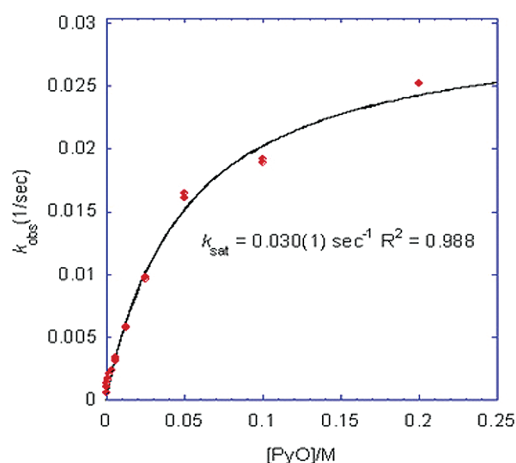
Figure 6. PyO dependence for the reaction of PyO with 2a in CH 3 CN at 298 K. Conditions were [Re] = 0.3 mM, [PyO] = 0.015 M–0.2 M. Data was fit with non-linear least-squares fitting to an equation describing saturation in [PyO]: k_{\text{obs}} = k'[\text{PyO}]/(k'' + [\text{PyO}]) .
