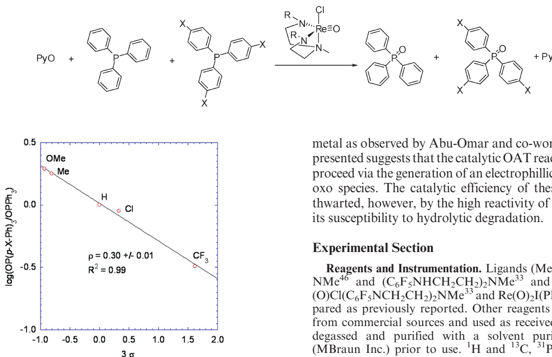
Figure 9. Hammett Plot obtained from competition experiments with para-substituted triaryl phosphines ( p -X-Ph) 3 P (X = OMe, Me, Cl, CF 3 ) as depicted in Scheme 4. The ratio of products was obtained by integration of the 31 P NMR spectrum for each experiment.
