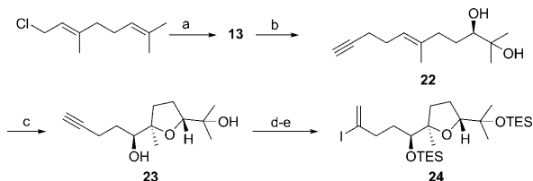
Scheme 5. Synthesis of the right-hand fragment. Reagents and conditions: a) 1-Trimethylsilylpropyne, n BuLi, THF, −78 °C, then Bu 4 NF, 88%; b) AD-Mix β, CH 3 SO 2 NH 2 , t BuOH, H 2 O, 53%; c) 18 , Oxone, K 2 CO 3 , Bu 4 NH 2 SO 4 , CH 3 CN, H 2 O, then Py-CSA, 83%, d.r. = 13:1; d) TESCl, imidazole, DMAP, DMF, 89%; e) Et 3 SiH, [CpRu(NCCH 3 ) 3 ]PF 6 , CH 2 Cl 2 , then I 2 , 2,6-lutidine, 82%. Cp = cyclopentadienyl, DMAP = 4-dimethylaminopyridine, Py-CSA = pyridinium camphorsulfonate, TES = triethylsilyl.
