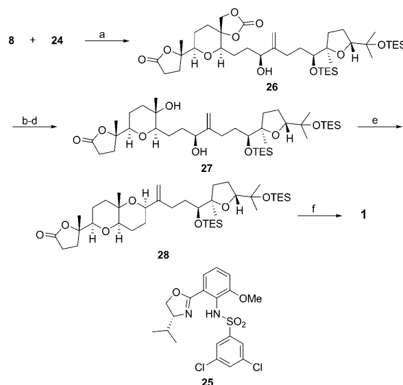
Scheme 6. Completion of the synthesis. Reagents and conditions: a) CrCl 2 , NiCl 2 ·DMP, 25 , Proton Sponge, Mn, Cp 2 ZrCl 2 , LiCl, CH 3 CN, 84%, d.r. = 8:1; b) K 2 CO 3 , MeOH, 91%; c) TsCl, Et 3 N, Bu 2 SnO, CH 2 Cl 2 , 92%; d) NaBH 4 , HMPA, 50 °C, 76%; e) Me 3 P=C(H)CN, C 6 H 6 , 80 °C, 40%; f) Bu 4 NF, THF, 77%. DMP = 2,9-dimethylphenanthroline, HMPA = hexamethylphosphoramide.
