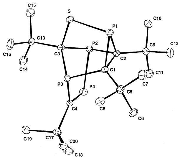
Fig. 11. Molecular structure of P_4SC_4Bu'_4 ( 13 ) together with the atomic numbering scheme and some selected bond lengths (Å) and bond angles (°). S–C(3) = 1.836(3), S–P(1) = 2.0939(13), P(1)–C(2) = 1.857(3), P(1)–C(1) = 1.861(3), P(2)–C(3) = 1.866(3), P(2)–C(2) = 1.875(3), P(2)–P(4) = 2.2133(11), P(3)–C(4) = 1.851(3), P(3)–C(3) = 1.877(3), P(3)–C(1) = 1.905(3), P(4)–C(4) = 1.692(3), C(1)–C(2) = 1.569(4), C(3)–S–P(1) = 95.71(9), C(2)–P(1)–C(1) = 49.93(11), C(2)–P(1)–S = 100.12(9), C(3)–P(2)–C(2) = 93.34(12), C(3)–P(2)–P(4) = 96.77(9), C(4)–P(3)–C(3) = 97.78(12), C(4)–P(4)–P(2) = 98.16(10), P(4)–C(4)–P(3) = 117.63(15).
