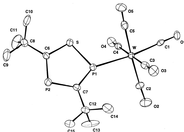
Fig. 7. Molecular structure of [\text{W(CO)}_5\eta^1\text{-P}_2\text{SC}_2\text{Bu}_2^t] ( 7 ) together with the atomic numbering scheme and some selected bond lengths (Å) and bond angles ( ^\circ ): \text{P(1)}-\text{S}=2.045(4) , \text{S}-\text{C(6)}=1.726(10) , \text{C(6)}-\text{P(2)}=1.690(11) , \text{P(2)}-\text{C(7)}=1.763(11) , \text{P(1)}-\text{C(7)}=1.695(11) , \text{P(1)}-\text{W}=2.483(3) , \text{W}-\text{C(1)}=2.014(11) , \text{P(1)}-\text{S}-\text{C(6)}=100.3(4) , \text{C(6)}-\text{P(2)}-\text{C(7)}=101.8(5) , \text{P(2)}-\text{C(7)}-\text{P(1)}=117.8(6) , \text{S}-\text{P(1)}-\text{W}=113.04(14) , \text{P(1)}-\text{W}-\text{C(1)}=173.2(3) .
