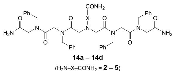
Fig. 4. Examples of the dimers isolated from the synthesized trial sequences
