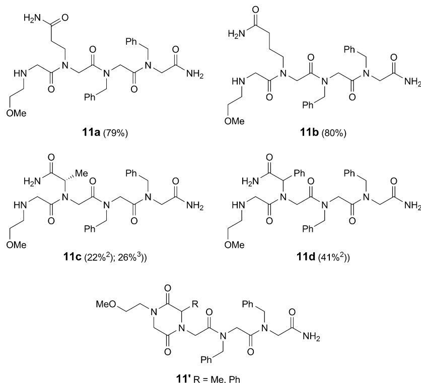
Fig. 3. Synthesized tripeptide sequences 11a – 11d and their yields after HPLC purification ( 11' is the diketopiperazine (DKP) side product)
