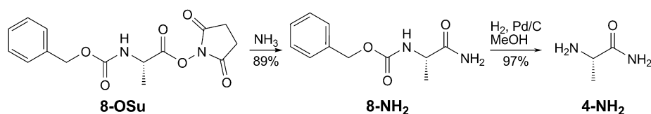
Scheme 3. Synthesis of Alaninamide (4-NH 2 ) as Free Amine . Su, N -Succinyl.
