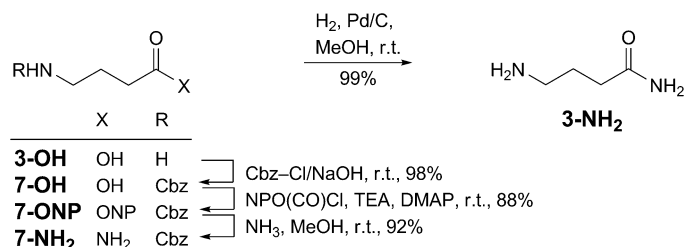
Scheme 2. Synthesis of 3-Aminopropanamide (3-NH 2 ) as Free Amine . Abbreviations: NP, 4-nitrophenyl; Cbz, (benzyloxy)carbonyl; TEA, Et 3 N; DMAP, 4-(dimethylamino)pyridine.
