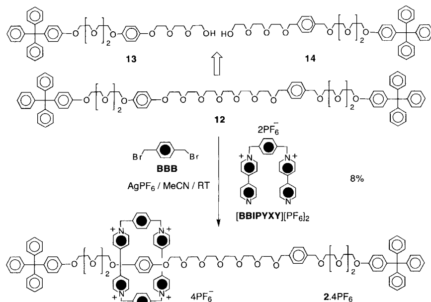
Scheme 3. Synthesis of [2]rotaxane 2 \cdot 4\text{PF}_6 .
