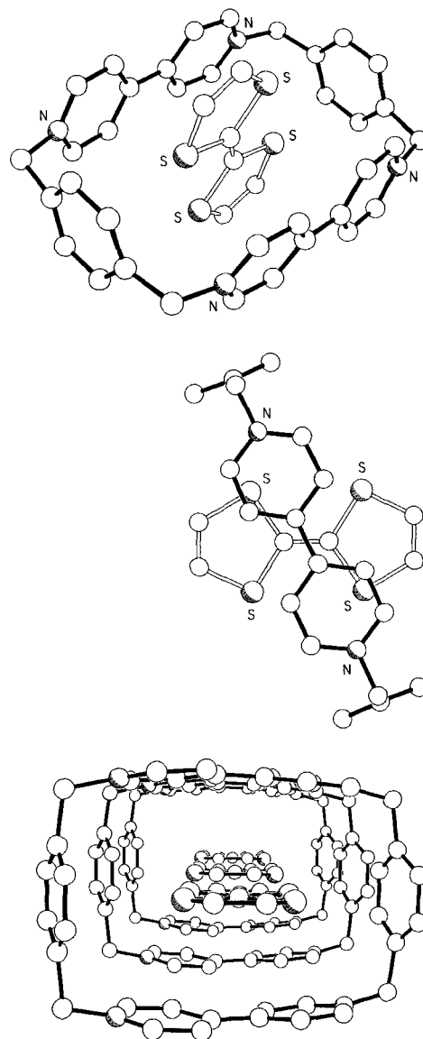
Figure 12. a) Ball-and-stick representation of the solid-state structure of [\text{BBIPYBIXYCY} \cdot \text{TTF}]^{4+} . b) Side-on and c) end-on views of the stepped stack-like superstructure of the 1:1 complex in one of the crystallographic directions.
