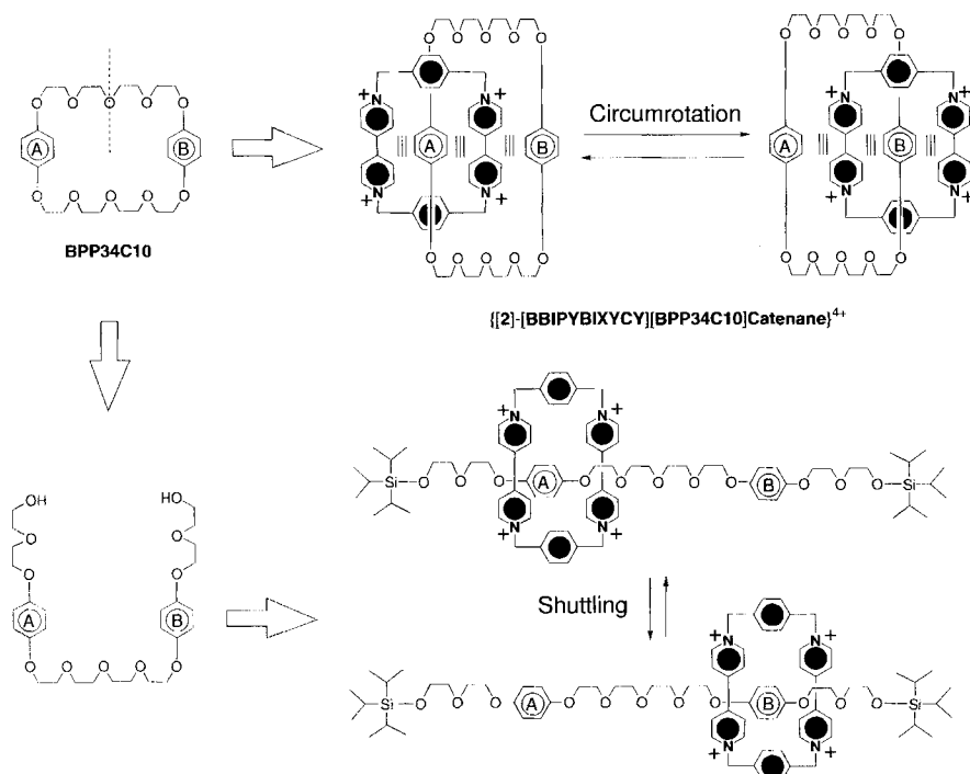
Figure 3. The analogy between the circumrotation of the tetracationic cyclophane component around the crown ether component in a [2]catenane and the possibility of a shuttling process in a [2]rotaxane that directed our attention toward the synthesis of a molecular shuttle.
