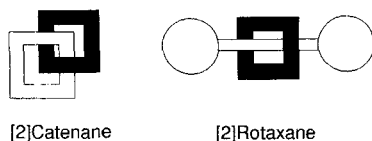
Figure 1. Schematic representations of a [2]catenane and a [2]rotaxane.
