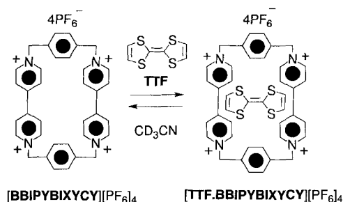
Scheme 10. Equilibrium between [\text{BBIPYBIXYCY}][\text{PF}_6]_4 and TTF in MeCN.
