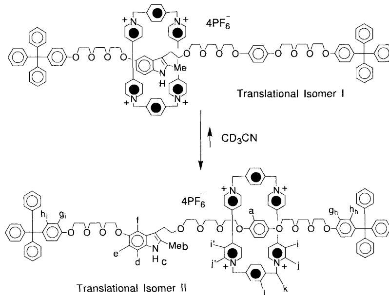
Figure 10. The translational isomers 1 and 2 and the labeling of the protons in the [2]rotaxane 3·4PF 6 .
