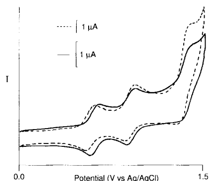
Figure 18. A comparison between the anodic cyclic voltammogram of the dumbbell-shaped compound 36 and the [2]rotaxane 4 ·4PF 6 .
