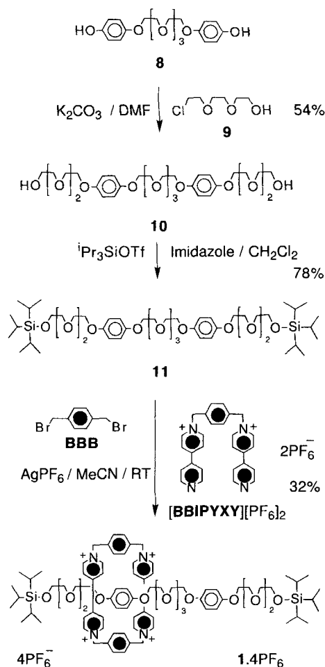
Scheme 2. Synthesis of [2]rotaxane 1·4PF 6 .
