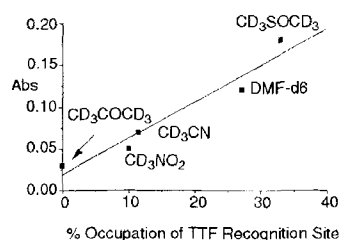
Figure 16. The relationship between absorbance (Abs) of the CT band at 750 nm and the percentage occupation of the translational isomers of the [2]rotaxane 4 \cdot 4\text{PF}_6 , determined by integration of the ^1\text{H} NMR spectra recorded in different solvents at room temperature.
