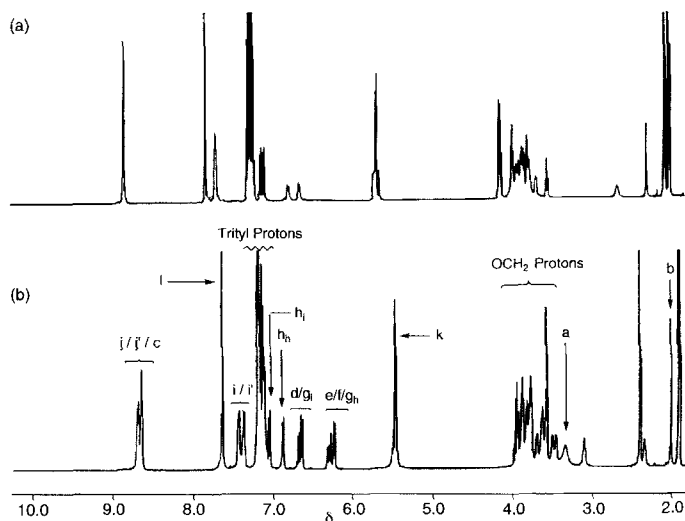
Figure 11. Variable-temperature 1 H NMR spectra of the [2]rotaxane 3·4PF 6 recorded in CD 3 CN at a) 343 K and b) 233 K.
