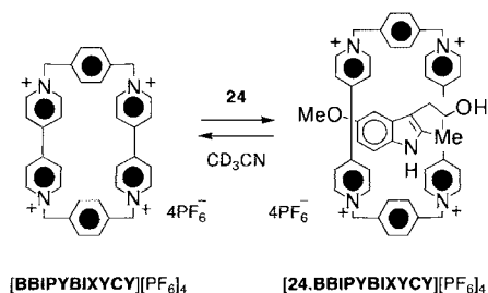
Scheme 5. Complexation of the model indole by cyclobis(paraquat- p -phenylene).
