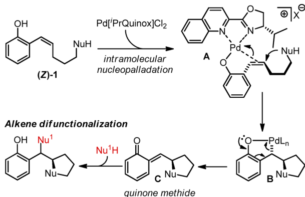
Scheme 1. Proposed Mechanism for Pd(II)-Catalyzed Alkene Difunctionalization via a Putative Quinone Methide Intermediate
