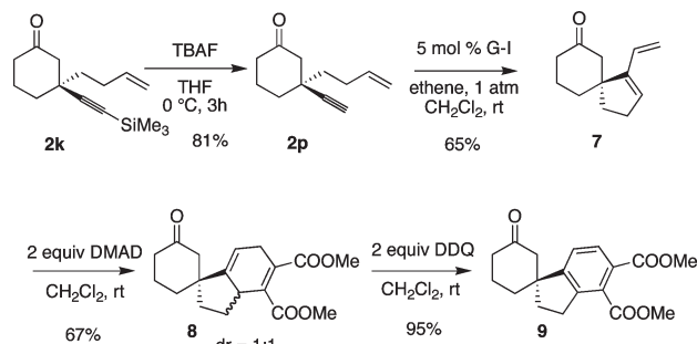
Scheme 4. Sequence Ene-Yne Methathesis/Diels–Alder/Aromatization Reaction
