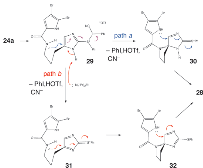
SCHEME 5. Mechanistic Speculation Governing the \text{PhI}(\text{CN})\text{OTf} -Mediated Tetracyclization of 24a
