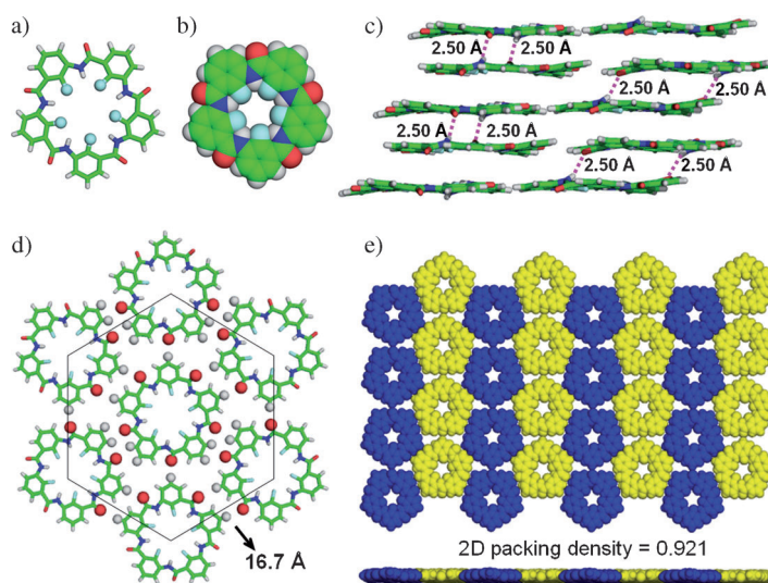
Figure 3. Crystal structure and 2D molecular packing of macrocyclic fluoropentamer 2 . a) Top view. b) CPK model of 2 built on the basis of van der Waals radii (H gray: 1.20; C green: 1.70; O red: 1.52; N blue: 1.55; F cyan: 1.47 Å). c) Formation of discrete pairs of isolated H bonds (2.50 Å) between two pentamers, which stabilize the interplanar stacking. d) Pseudo-hexagonal arrangement with a side length of 16.7 Å and with each pentagon forming two edge-to-vertex and two smaller and two larger edge-overlap contacts with its six close neighbors. Small spheres represent partially charged “sticky” hydrogen (gray) and oxygen (red) atoms that are involved in C=O...H–C H bonds, which allow tight packing of pentagonal molecules. e) Top and side views of alternating striped lattice packing, consisting of pentagons pointing in opposite directions in CPK model, which reproduces the densest mathematical crystal formed by pentagons (Figure 1b). The average interplanar distance is 3.1 Å. The 2D packing density of 0.921 was calculated by using the van der Waals radii specified in (b).
