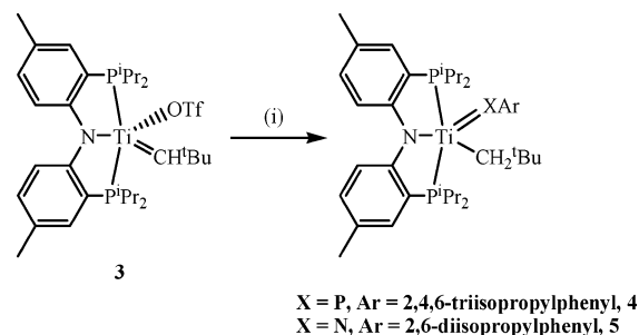
Scheme 2. Formation of Phosphinidene 4 and Imido 5 from 3 a
