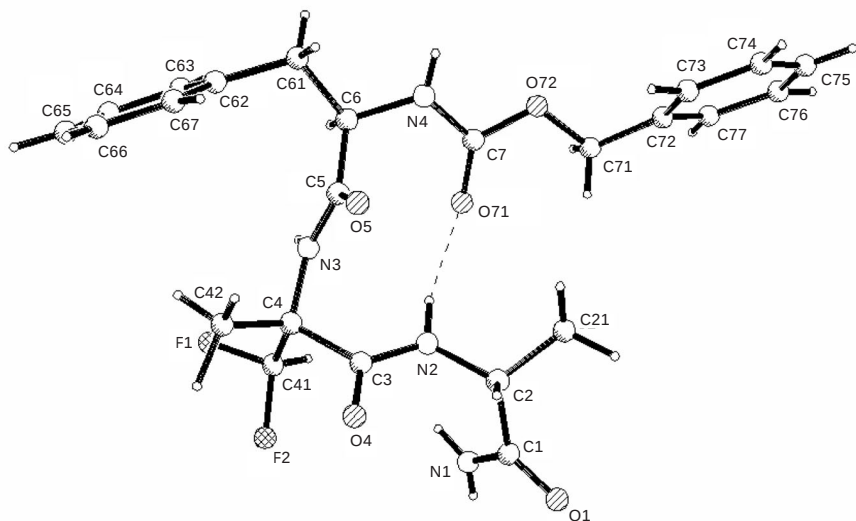
FIG. 3 Molecular structure of Z-(R)-Phe-(R)-(α-Dfm)Ala-(R)-Ala-NH 2 ( 7c/1 )
