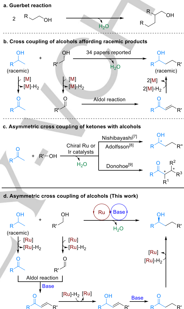
Figure 1. Guerbet reaction, cross coupling of ketones with alcohols and cross coupling of alcohols via hydrogen autotransfer.
