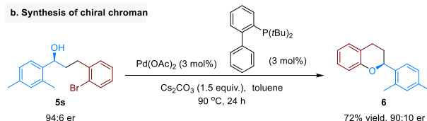
Figure 3. Gram-scale reaction and synthetic applications.
